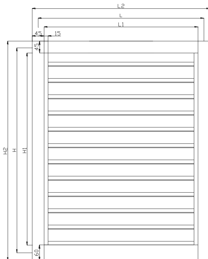
FA-450 – ΟΨΗ (L x H)
