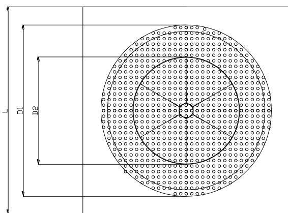
SW-1400-P-C – ΟΨΗ
