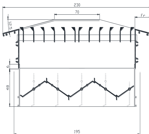
TL-202-2-D/212-2-D – TOMH ME DAMPER (L x 195 mm)
